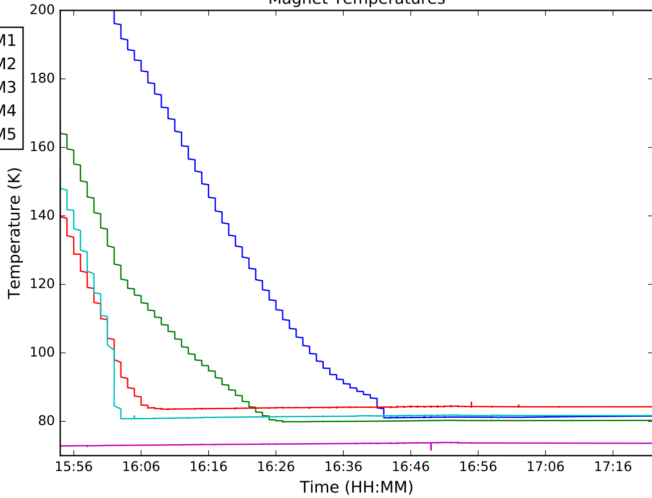
Magnet Temperatures
